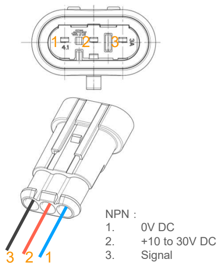
Dia. 22.2 Divider Monitoring Sensor Wiring Connection
