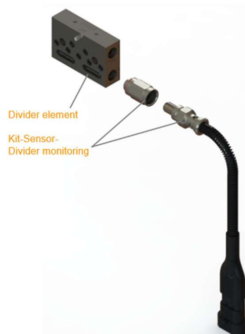
Dia. 13.2 Example for (ME) Middle element with Kit-Sensor divider monitoring on the right side
