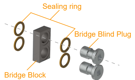
Dia. 18.1 Bridge without Outlet
