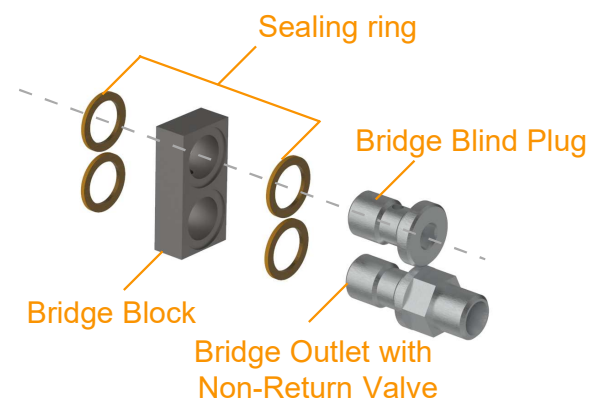
Dia. 18.2 Bridge with Outlet and Non-Return Valve
