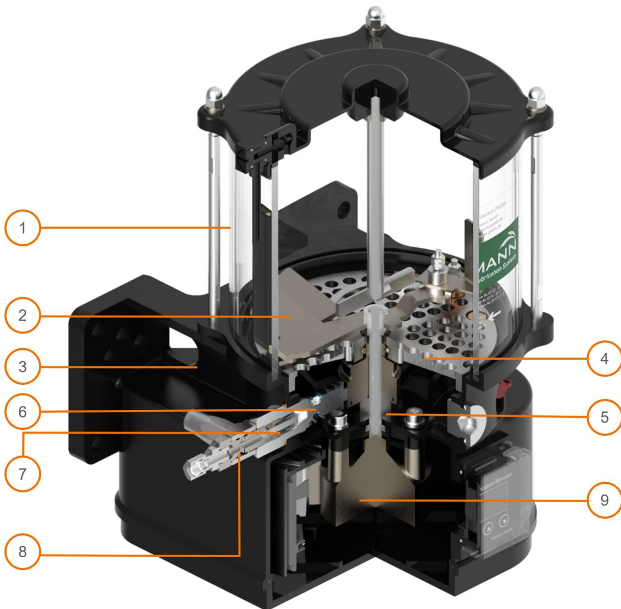
Dia. 13.1 Pump working principle
