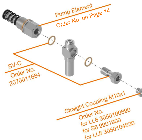
Dia. 16.2 Explosion for SV-C with PE + Straight Coupling
