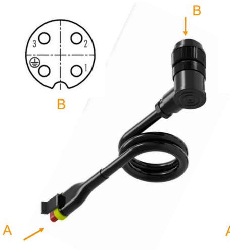
Dia. 17.2 Cable kit-divider monitoring-with BD-plug
