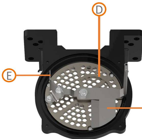
Dia. 20.1 Low level indication perspective representation
