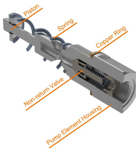
Dia. 14.2 Pump Element structure
