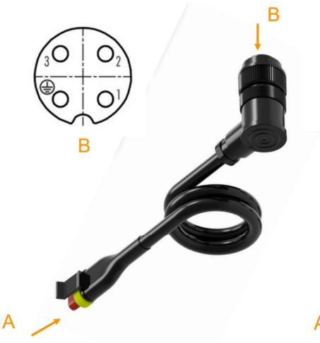
Dia. 17.2 Cable kit-divider monitoring- with BD-plug
