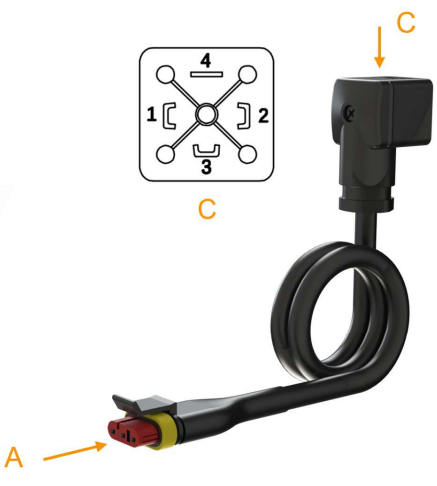
Dia. 17.3 Cable kit-divider monitoring- with HSC-Plug
