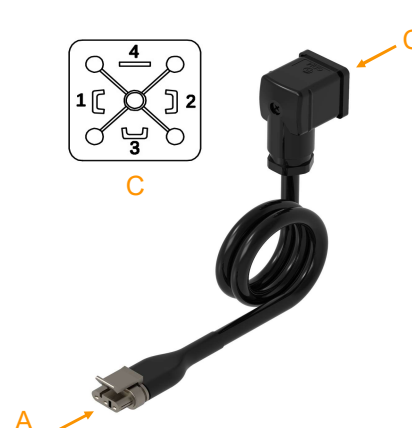
Dia. 23.3 Cable kit- divider monitoring with HSC plug
