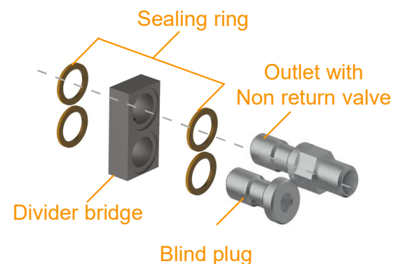
Dia. 18.2 Kit-Divider bridge with Outlet and Non-Return Valve
