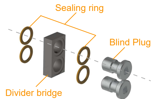
Dia. 18.1 Kit-Divider bridge without Outlet
